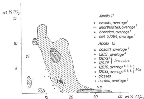
Fig. 5. TiO 2 versus Al 2 O 3 contents of glasses, igneous rocks, breccias and soil from Apollo 11 and Apollo 12. Glass analyses of this work (Apollo 12) are represented by dots. All hatched areas comprise 222 data points of Apollo 11 glass analyses taken from LEVINSON, Vols. 1 and 2 (1970). The narrow-hatched areas comprise the indicated percentages of all data points. References for all other data are designated by superior numerals and listed in caption of Fig. 8.
